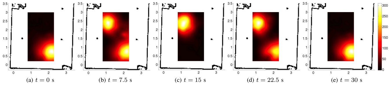
Fig. 8. Spatially distributed light intensity variations. Axis in metres.
