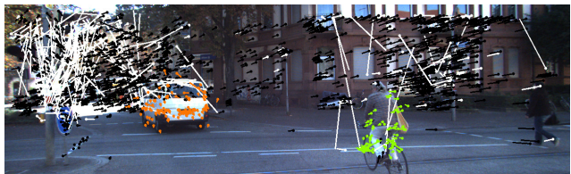
Fig. 3: Sparse optical flow vectors grouped by motion. Static points are shown in black, while the dynamic points are coloured by their cluster assignment. Points with low density in motion space (considered noise) are marked in white.
