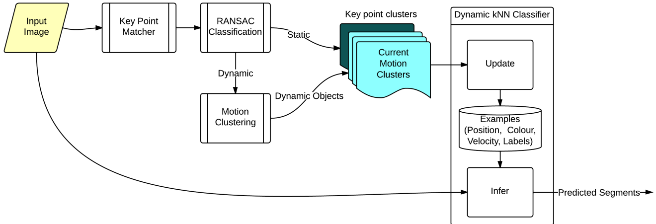
Fig. 2: An overview of the object extraction and learning process used in this paper.
